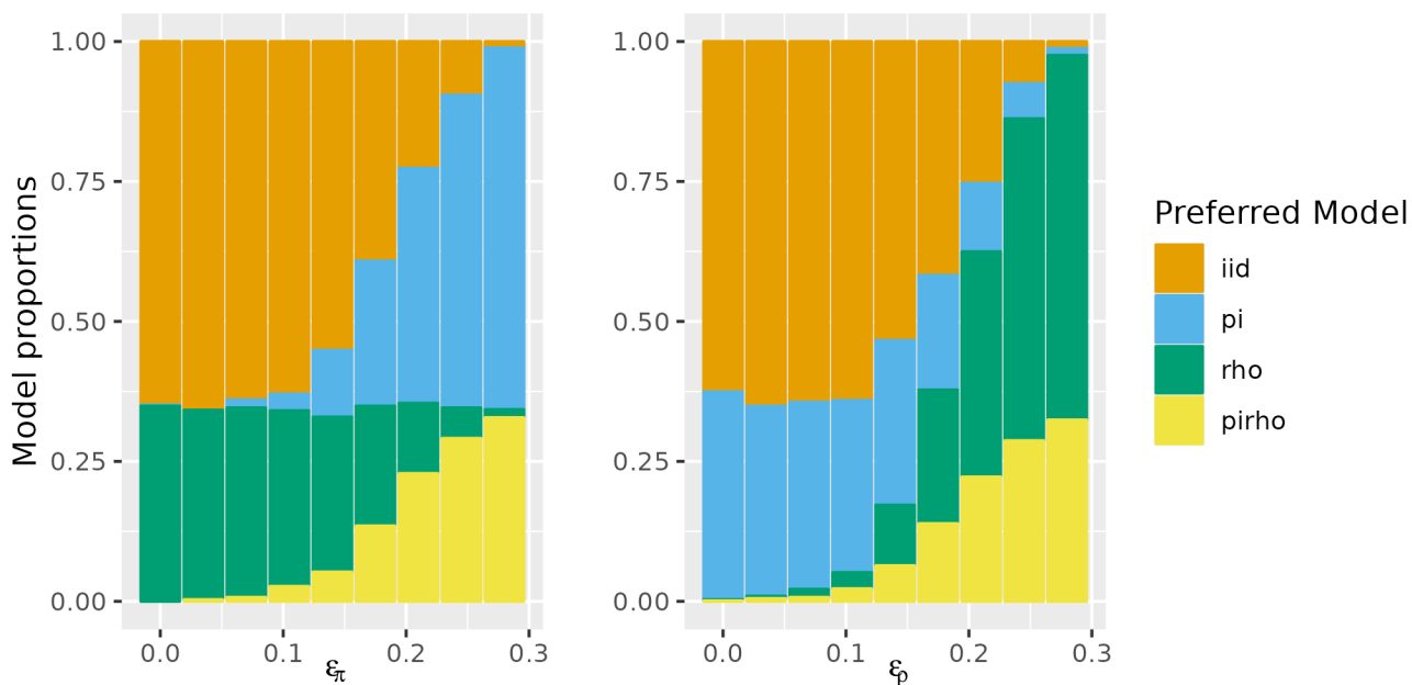
Figure 4.2: Plot of preferred model in function of \epsilon_\pi and \epsilon_\rho
