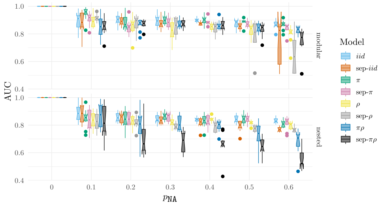
Figure 3.5: AUC in function of p_{NA} , the proportion of missing links for various colBiSBM models and their LBM counterparts
