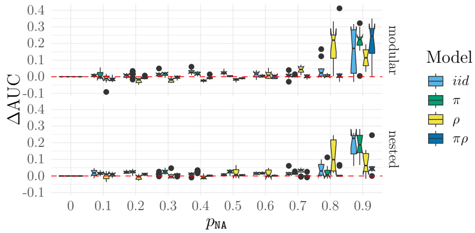
Figure 3.5: \Delta\text{AUC} in function of p_{\text{NA}} . The dashed red lines indicate the value 0 for which \text{AUC}_{LBM} = \text{AUC}_{\text{colBiSBM}}
