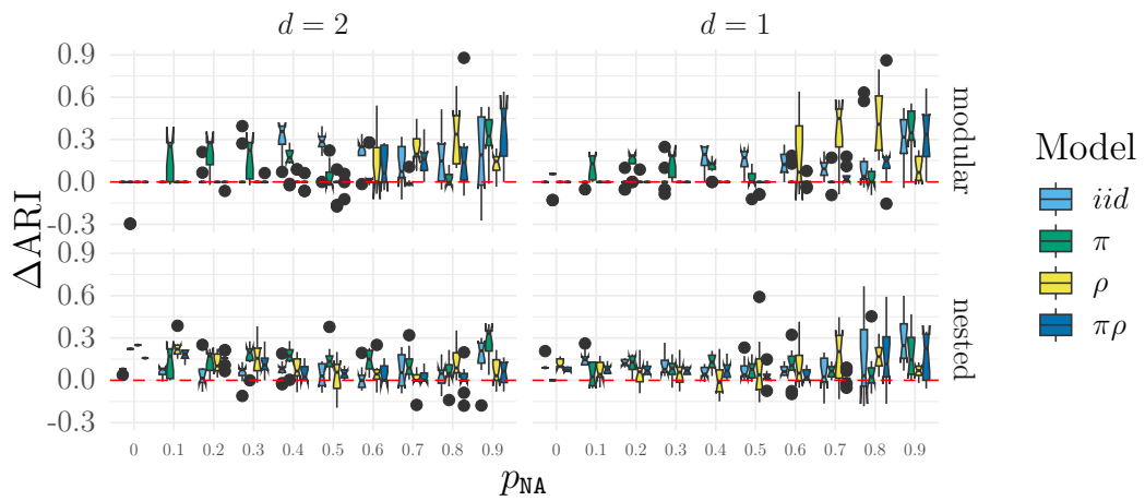
Figure 3.6: \Delta\text{ARI} in function of p_{\text{NA}} . The dashed red lines indicate the value 0 for which \text{ARI}_{LBM} = \text{ARI}_{\text{colBiSBM}}
